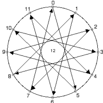
Figure 1. Circle of fourths in the 12-tempered system.
