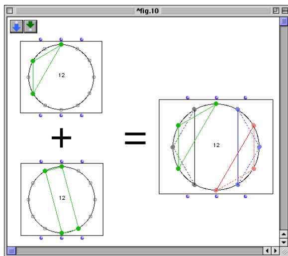
Figure 10: factorisation of \mathbb{Z}/12\mathbb{Z} in two subsets.
