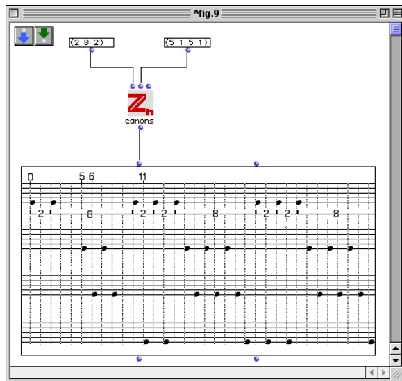
Figure 9: a tiling rhythmic canon .
