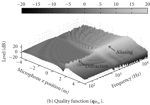
FIGURE 4: Frequency responses ( \mathbf{w}_{\Psi_m} ) and quality function ( \mathbf{q}_{\Psi_m} ) of an 8 m, 48-channel, loudspeaker array simulated on a line at 2 m from the loudspeaker array for synthesis of a source of degree -2 (far source of Figure 3).
