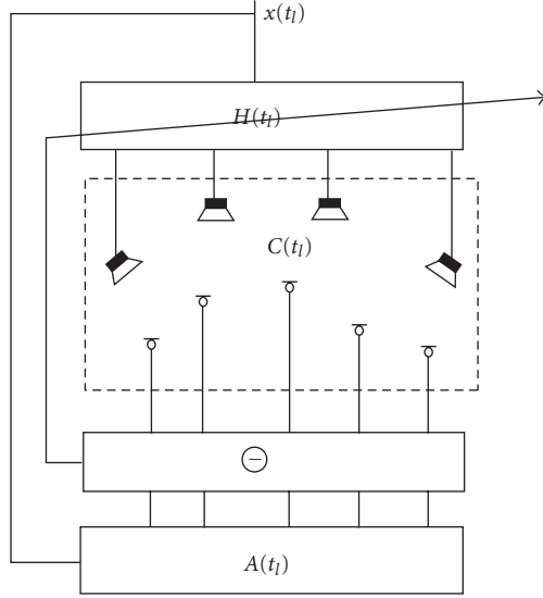
FIGURE 6: Equalization for sound reproduction.
