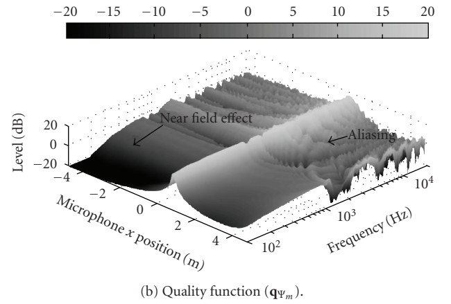
FIGURE 5: Frequency responses ( \mathbf{w}_{\Psi_m} ) and quality function ( \mathbf{q}_{\Psi_m} ) of an 8 m, 48-channel, loudspeaker array simulated on a line at 2 m from the loudspeaker array for synthesis of a source of degree +2 (close source of Figure 3).
