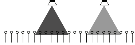
FIGURE 7: Measurement selection for individual equalization.
