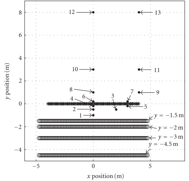
FIGURE 11: Top view of the considered system: 48 regularly spaced (16.75 cm) loudspeakers (*) measured on 4 depths ( y = -1.5, -2, -3, -4.5 m) with 96 regularly spaced (10 cm) microphones (circle) reproducing 13 test sources (dot).
