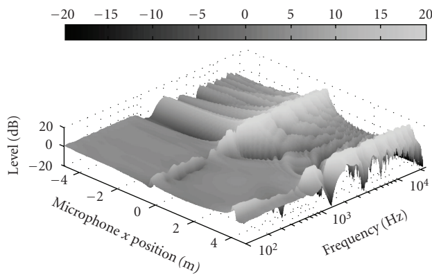
(b) Quality function ( q_{\Psi_m} ) for close source of Figure 3.
