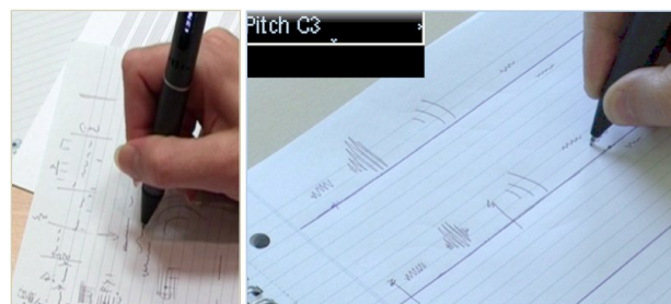
Livescribe pens run Java ME programs ( penlets ) and offer a range of functions, including auditory and visual feedback, audio recording and replay, interactive buttons and special areas printed on paper. For example, Figure 5 shows boxes with multiphonic tones for a saxophone piece that MB printed from OpenMusic . This let MB reflect on each sound while working on paper, using a penlet to replay sounds at will.
