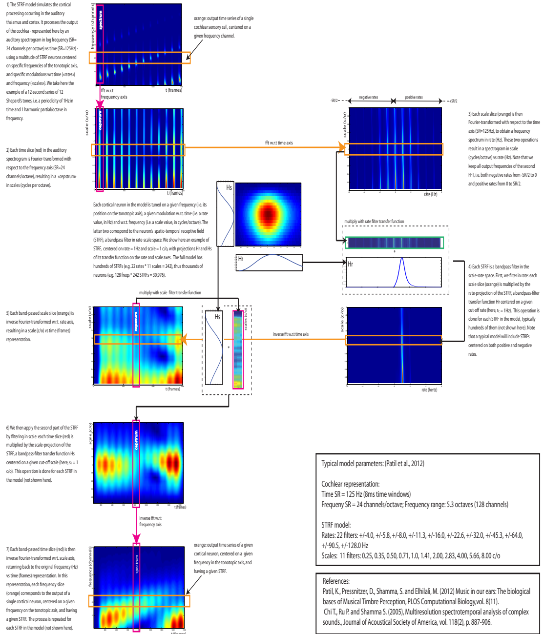
FIGURE 2.2 – Shamma's STRF model : a signal processing primer.
